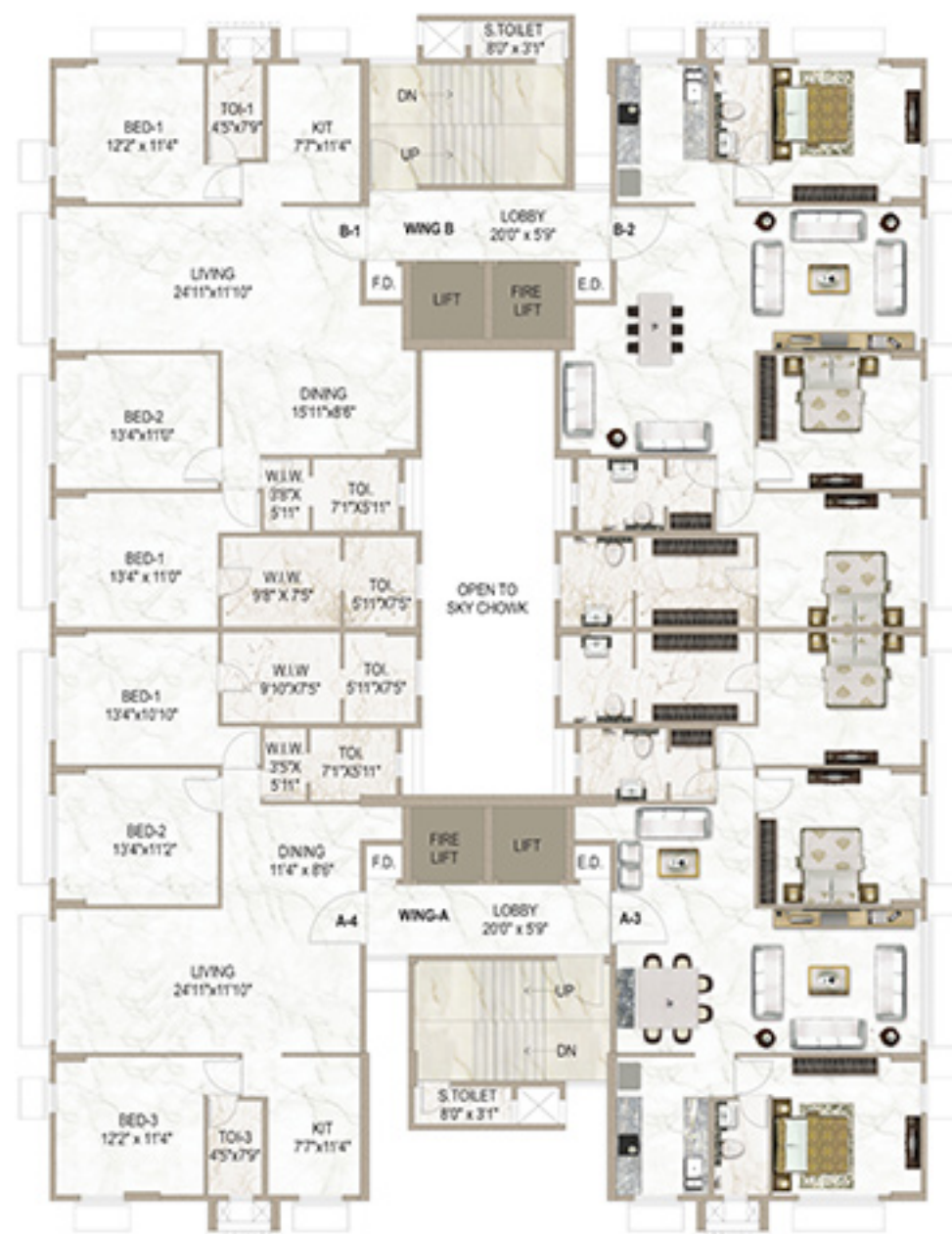
10th Floor Plan
