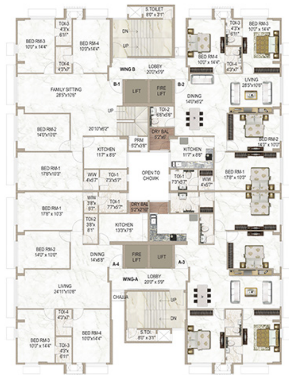
14th Floor Plan
